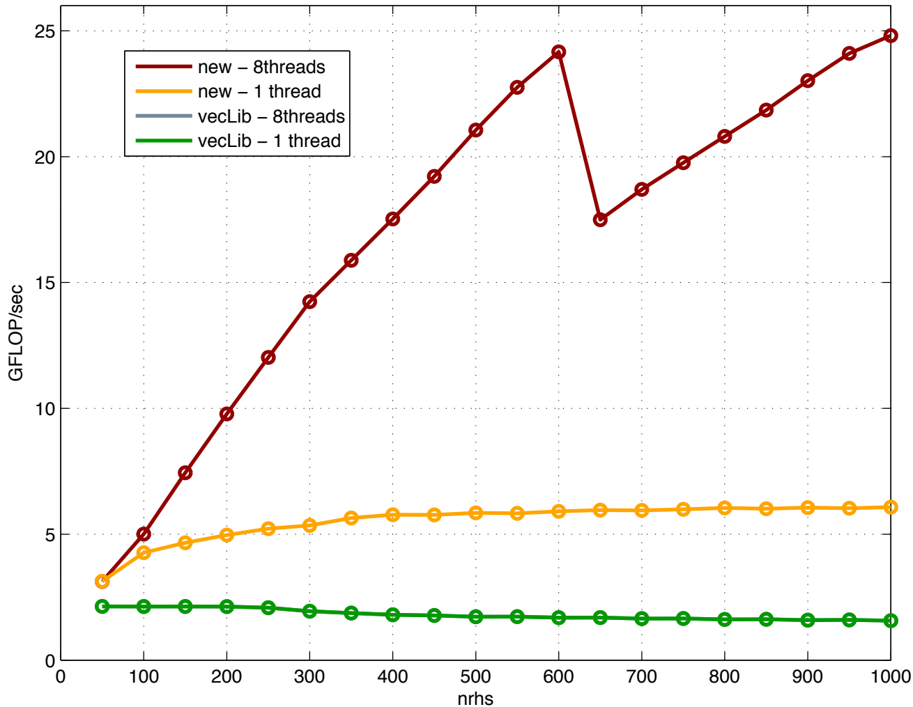
LDLT Solve (DSYTRS), N=4000, VecLib Processor 2 x 2.26GHz Quad-Core Intel Xeon
