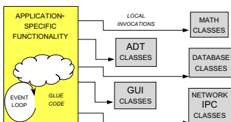
(A) CLASS LIBRARY ARCHITECTURE
