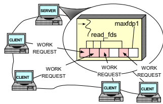
(1) ITERATIVE SERVER
