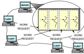
(2) CONCURRENT SERVER
