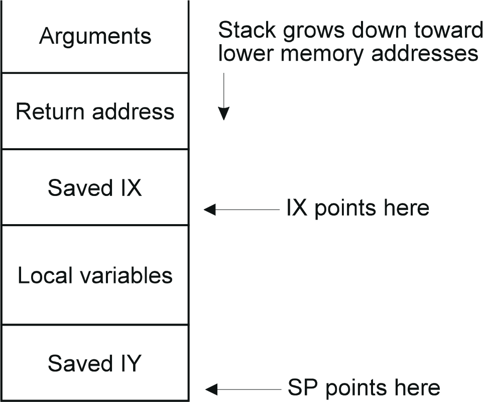
Figure 4-1; Stack frame
