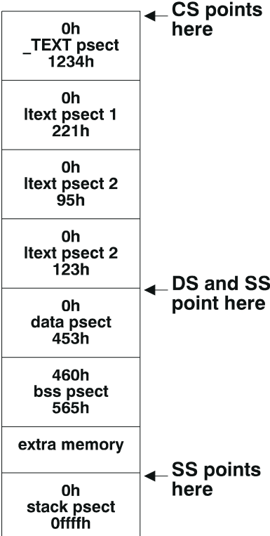
Figure 4-5; Large model memory layout
