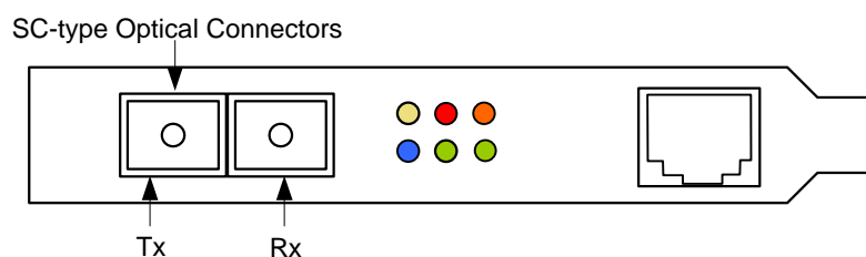
Figure 2-1. DAG 4.2S Card SC-type Optical Connectors.
